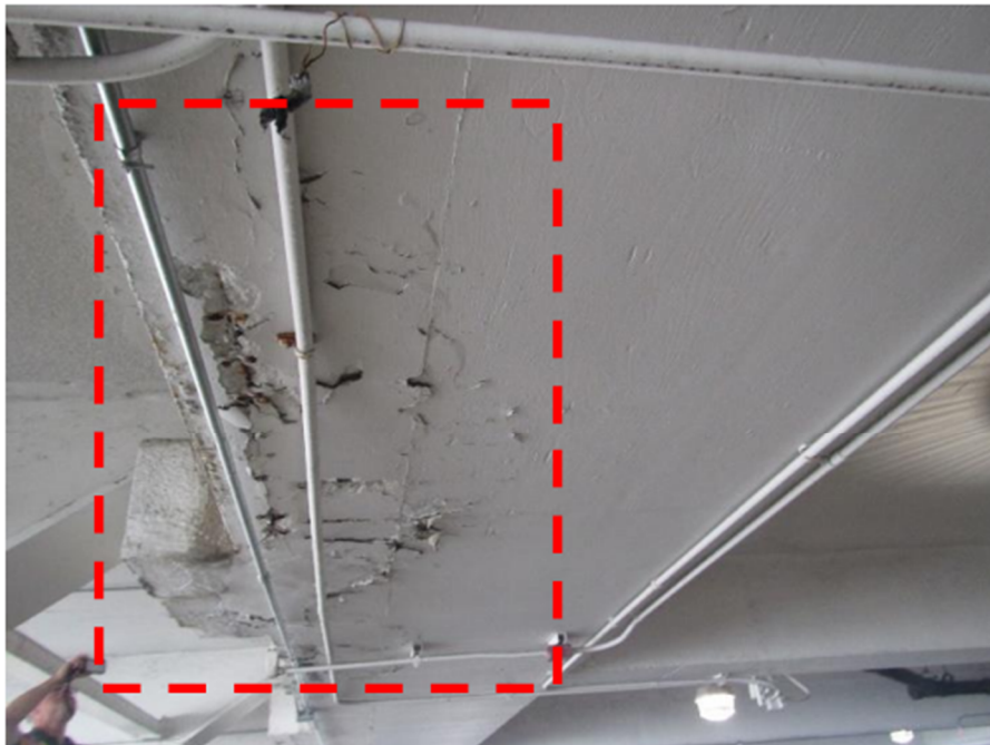
27 Spalled concrete and exposed reinforcement at underside of parking garage beam
