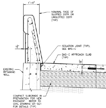
Proposed SSTR Retrofit at Retaining Wall
