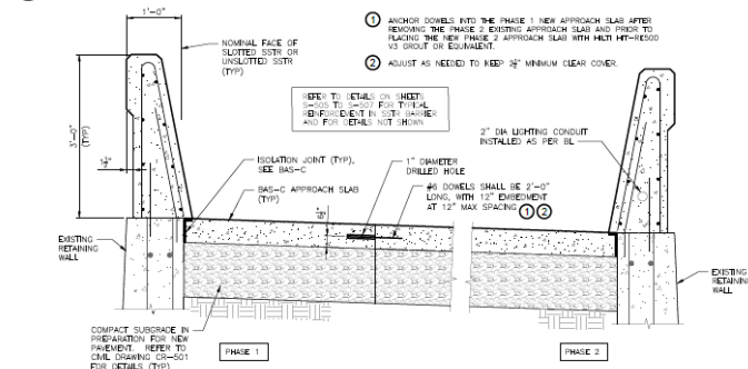
8 FINAL BRIDGE STRUCTURE - EAST APPROACH SLAB SHOWN (SOUTH APPROACH SLAB SIMILAR) 1"=1'-0"
