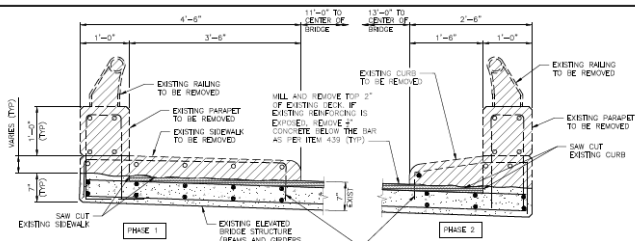
4 EXISTING BRIDGE STRUCTURE - DEMOLITION DETAIL 1"=1'-0"
