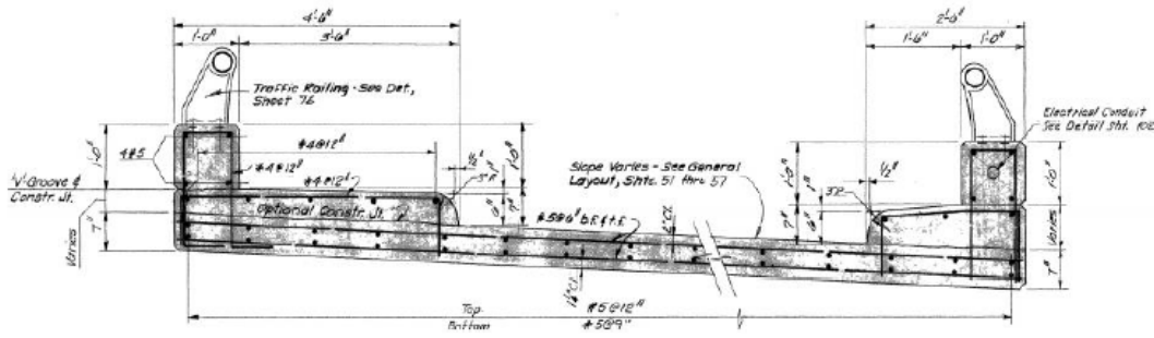
Existing Bridge Structure Deck Section
