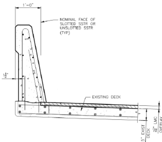
Proposed SSTR Retrofit at Bridge Structure
